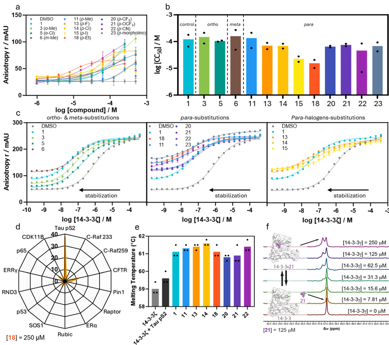
Fig. 3 a Dose-response fluorescence anisotropy data of compound titrations to 10 nM FITC-labeled Tau pS2 peptide and 100 nM 14-3-3ζ. Background (without 14-3-3ζ) subtracted, overnight measurement, mean and SD of technical duplicate (see ESI† Fig. S5 for another replicate). b Bar plot representation of CC_{50} values of the compound titrations shown in (a), mean and SD of scientific duplicate. c Dose-response fluorescence anisotropy data of 14-3-3ζ titrations to 10 nM FITC-labeled Tau pS2 peptide and 250 μM compound, mean and SD of technical duplicate (see ESI† Fig. S6 for another replicate). d Radar plot of stabilization factors at 250 μM compound 18 (SF 250 ) from 14-3-3ζ FA protein titrations with 10 nM (Tau pS2 peptide) or 100 nM (13 other peptides) FITC-labeled peptide. Mean of three individually performed experiments (see ESI† Fig. S8 for the protein titrations). e Differential scanning fluorimetry assay results. Identified melting temperatures ( T_m ) of 14-3-3γ alone (2.5 μM) and in the presence of Tau pS2 peptide (25 μM) and additionally with selected compounds (75 μM). Mean of three individually performed experiments. f 19 F-NMR spectra (565 MHz, 298 K, 10 vol% D 2 O in H 2 O) of compound 21 (125 μM) at varying concentrations of 14-3-3γ (0–250 μM) indicates ligand binding to 14-3-3γ.
