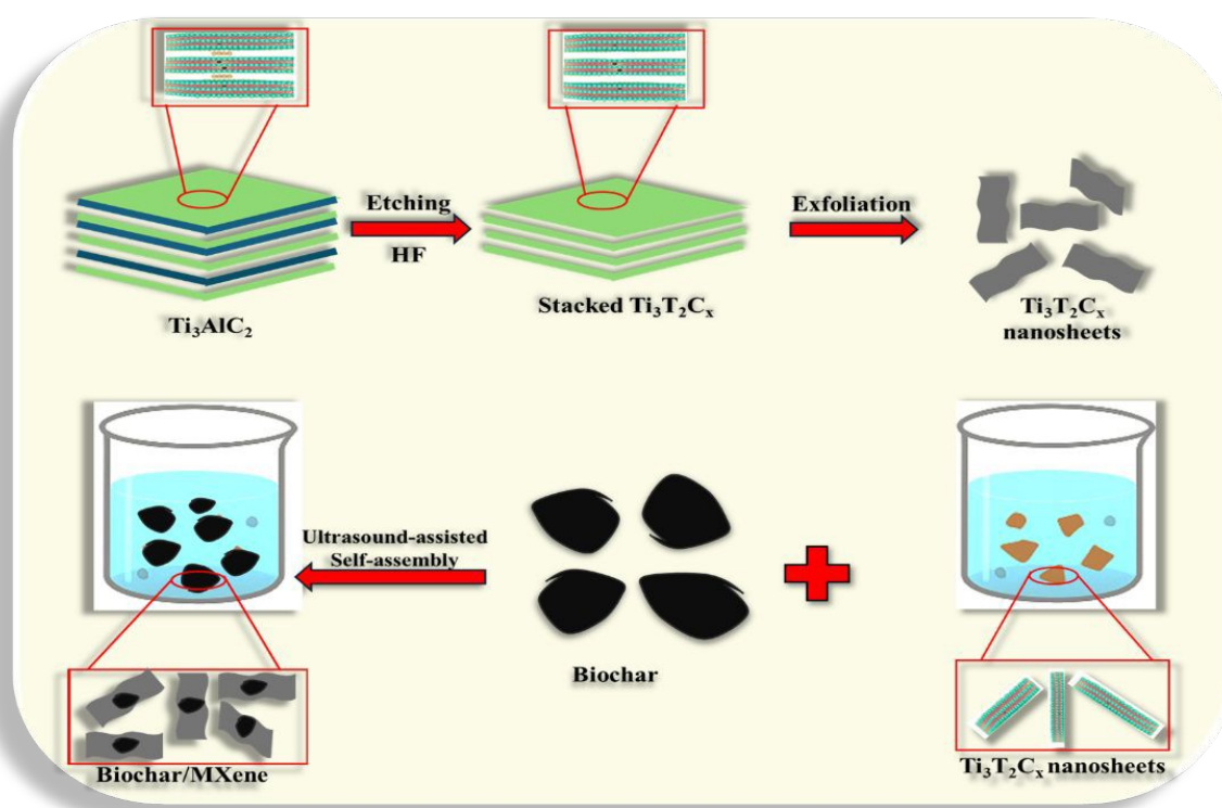
Figure 8. Biochar/MXenes fabrication strategy.
