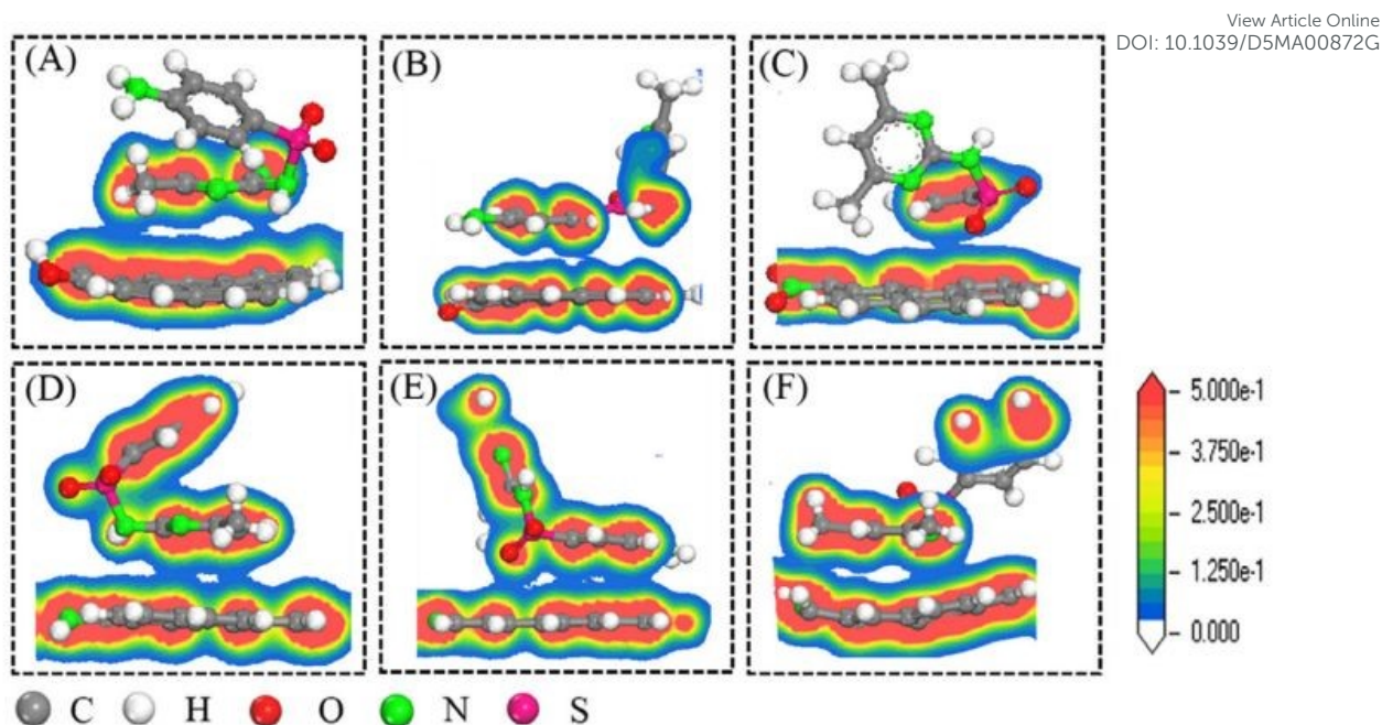
Figure 10. Charge density images showing SMT adsorption on functionalized MCB surfaces: (A) MCB-OH, (B) MCB-COOH, (C) MCB-NO 2 , (D) MCB-NH 2 , (E) C 5 H 5 N-MCB, and (F) C 4 H 5 N-MCB (Reproduced from reference [239] with permission from Elsevier, copyright 2019).
