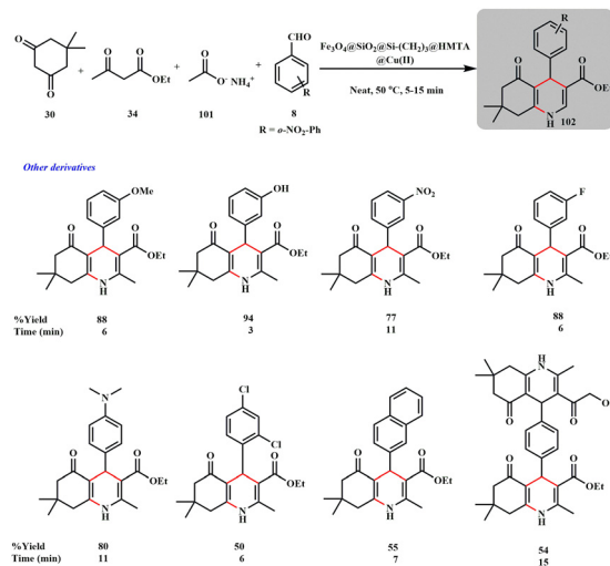
Scheme 46 Catalytic synthesis of hexahydroquinoline derivatives using an Fe 3 O 4 @SiO 2 @Si-(CH 2 ) 2 @HMTA@Cu nanocomposite (Salem et al. ).
