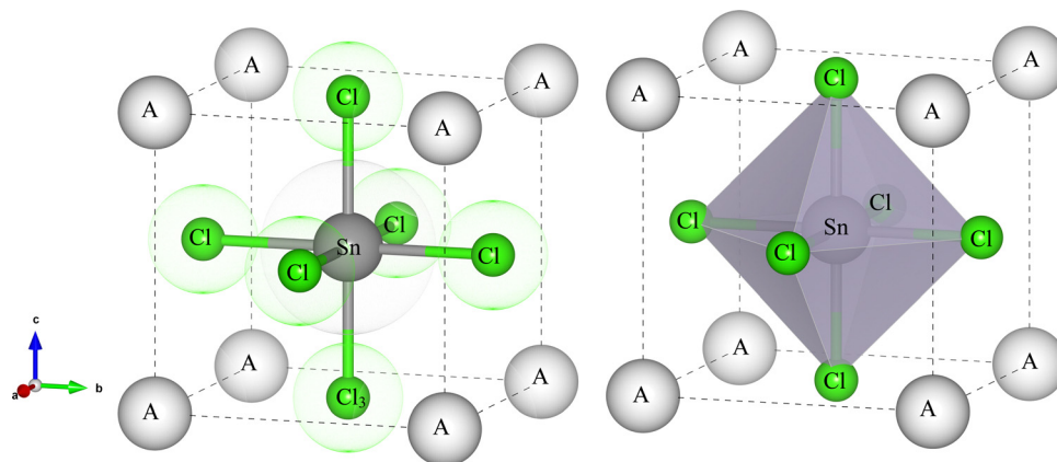
Fig. 1 The crystal structure of \text{ASnCl}_3 (A = Ga, In, and Tl).
