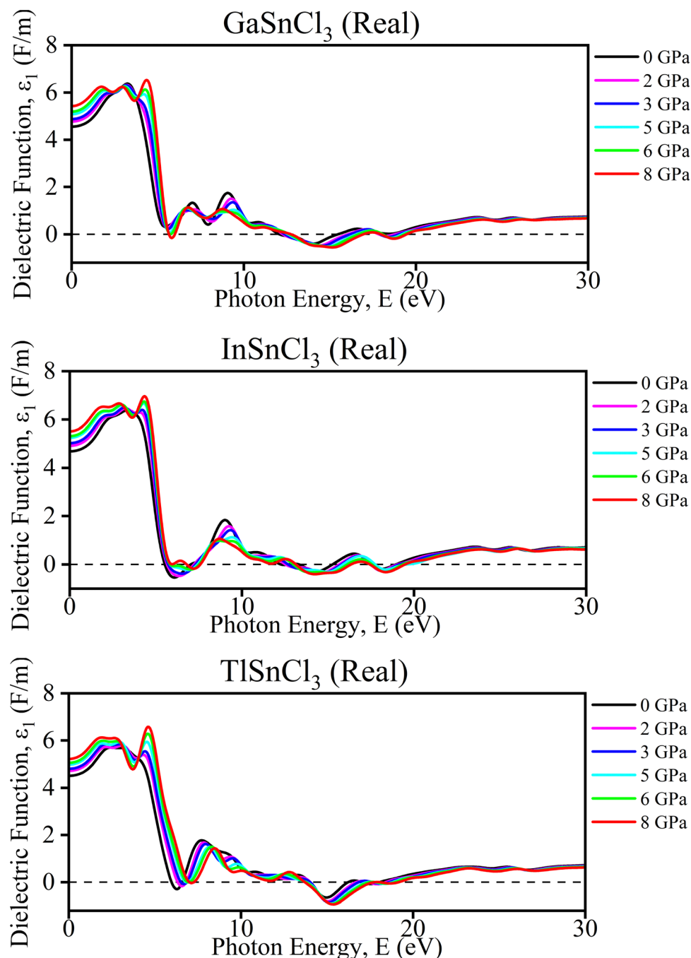
Fig. 10 Calculated pressure induced real spectra of dielectric function ( \epsilon_1 ) for \text{ASnCl}_3 ( A = \text{Ga}, \text{In}, \text{and Tl} ).
