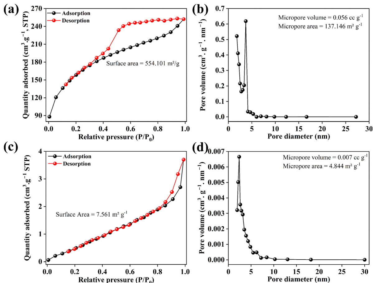
Fig. 2 BET analysis: (a) and (c) demonstrate N_2 adsorption–desorption isotherms, and (b) and (d) BJH pore size distribution of KZAC and PZC, respectively.
