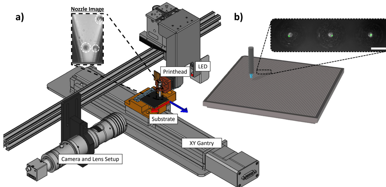
Fig. 1 a) An imaging module containing a camera and long working distance zoom lens is fixed in-line with the printhead, an LED positioned behind the printhead provides an illumination source. The camera continuously monitors the events within the glass nozzle of the printhead capturing a nozzle image after every dispensed droplet. The inset shows an example image of the nozzle (scalebar represents 50\ \mu\text{m} ), the cells within the nozzle are highlighted by white circles. The target labware is mounted on an XY gantry stage via bespoke holders. b) During instrument operation, the designated print area is scanned via a raster pattern below the nozzle. The printhead operating in drop-on-demand mode dispenses droplets into each well. A machine vision algorithm monitoring for cell dispensing events within the nozzle will provide feedback to the instrument to optimize single cell yield into the substrate. The inset zooming into the substrate shows a microscopy image of three example wells after cell printing. The dispensed cells are stained with CFSE and are shown in the green channel of the image. Reflected light imaging shows the features of the substrate in the gray channel. Scalebar represents 200\ \mu\text{m} .
