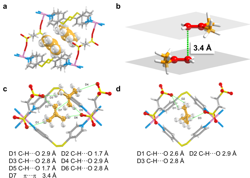
Fig. 3 (a) 2 \text{iso-C}_4\text{H}_8 molecules adsorbed in one pore cage of ZU-603 as revealed by single crystal analysis; (b) the packing diagram of 2 \text{iso-C}_4\text{H}_8 molecules adsorbed within one pore cage of ZU-603 as revealed by single crystal analysis; (c) the specific binding sites of \text{iso-C}_4\text{H}_8 on ZU-603 as revealed by single crystal experiments; (d) the specific binding sites of \text{iso-C}_4\text{H}_{10} on ZU-603 as revealed by DFT-D calculations (color code: silver, C; white, H; red, O; blue, N; yellow, S; pink, Cu; orange, C of the adsorbed molecules).
