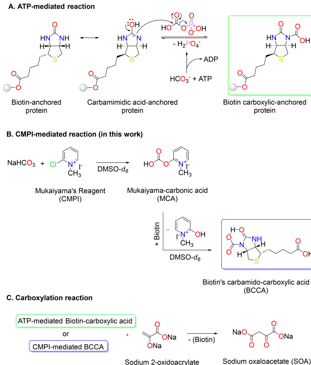
Scheme 1 A. Reaction mechanism of \text{CO}_2 transfer to biotin, forming biotin-carboxylic acid as a coenzyme. 2,14 B. The reaction of sodium bicarbonate as a C1-feedstock with 2-chloro-1-methylpyridinium iodide (CMPI) produces the Mukaiyama-carbonic acid (MCA) adduct, which subsequently reacts with biotin to form biotin's carbamido-carboxylic acid (BCCA), featuring a hydrogen atom between the two oxygen atoms that participates in an intramolecular hydrogen bond. This reaction is driven by CMPI, which functions as an oxygen-sink promoter. C. Conversion of sodium 2-oxidoacrylate to sodium oxaloacetate (SOA) through ATP- or CMPI-mediated formation of carboxylate/carboxylic biotin adducts.
