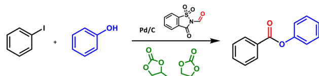
Scheme 18 Pd/C-catalysed phenoxycarbonylation of aryl iodides using DACs as the solvent. 127
