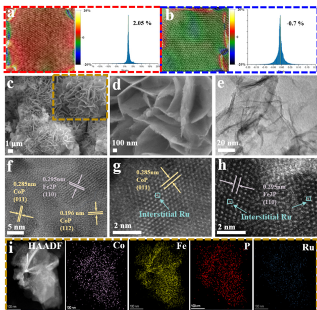
Fig. 1 (a and b) GPA (geometric phase analysis) test of FeCoP/FF-Q and FeCoP/FF-C electrodes. (c and d) SEM images of Ru-FeCoP/FF. (e) TEM image of powders on the surface of the Ru-FeCoP/FF electrode. (f) HRTEM images of powders on the surface of the Ru-FeCoP/FF electrode. (g and h) HAADF-STEM images of powders on the surface of the Ru-FeCoP/FF electrode. (i) EDX elemental mappings of powders on the surface of the Ru-FeCoP/FF electrode.
