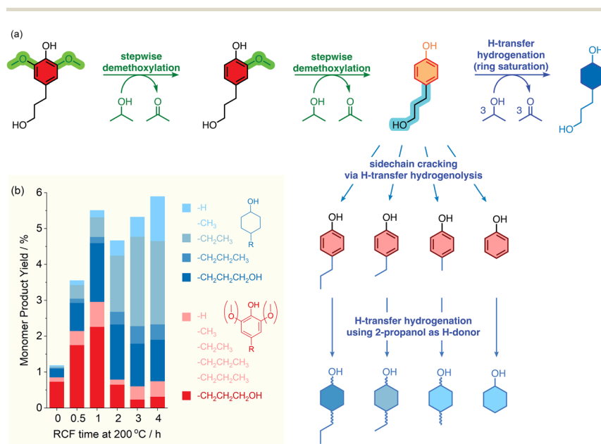
Scheme 1 (a) Proposed reaction network for HT-RCF over RANEY® Ni using 2-propanol as the H-donor. Lignin fragments undergo selective HDO, forming dihydrolignols, which then undergo stepwise demethoxylation (syringyl \rightarrow guaiacyl \rightarrow phenolic intermediates), after which H-transfer hydrogenation saturates the aromatic ring to give alkyl-substituted cyclohexanols. In parallel, the aryl propyl sidechain can shorten by H-transfer-hydrogenolysis, so the initially dominant formation of 4-(3-hydroxypropyl)cyclohexanol can diverge to the generation of ethyl phenol and 4-ethylcyclohexanol at longer times (main product when using fresh catalyst). 9,32,36,37,44,45 Note that the H-transfer saturation of syringyl and guaiacyl intermediates to the corresponding 2,(6)-(di)methoxy-4-alkyl-cyclohexanols is unlikely to take place in the presence of RANEY® Ni using 2-propanol as the H-donor. 29,38 (b) Time-resolved evolution of monomer yields during HT-RCF of post-consumer cardboard. Stacked bars show total monomer yield (GC-FID/MS) at 200 °C as a function of reaction time. Colours distinguish intermediate phenols (red scale) from cyclohexanol products (blue scale), further resolved by side-chain substituent at R (legend). (b) Shows that HT-RCF of cardboard at 200 °C begins producing phenolic monomers during heat-up, which peak within 1 h and then decline as they convert into alkyl phenols. With longer times, aromatic saturation dominates, yielding cyclohexanols, shifting from 4-(3-hydroxypropyl)cyclohexanol early to 4-ethylcyclohexanol after 3–4 h.
