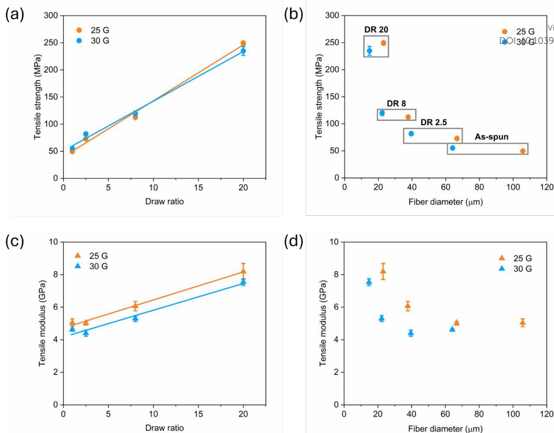
Figure 6. Tensile strength (top) and modulus (bottom) of 25 G and 30 G lignin-PVA fibres hot-drawn to a series of draw ratios.
