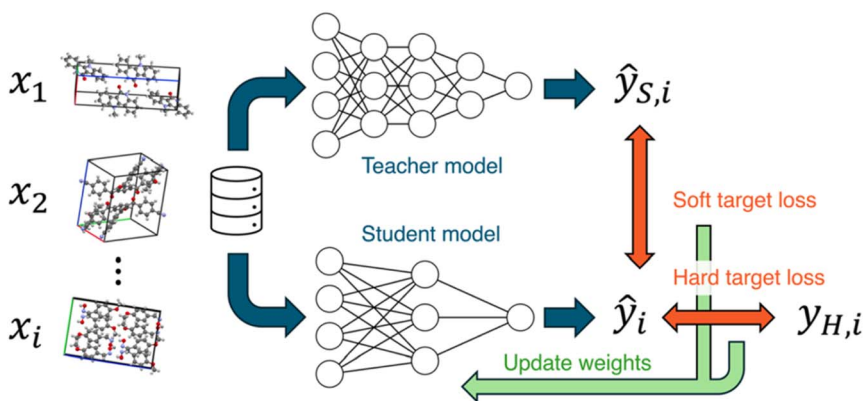
Fig. 5 Knowledge distillation of neural networks. In this work, the teacher and student models were the two neural network potentials, PreFerred Potential (PFP) and Crystal Hamiltonian Graph Network (CHGNet), respectively. Reproduced from https://doi.org/10.1039/d4fd00090k .
