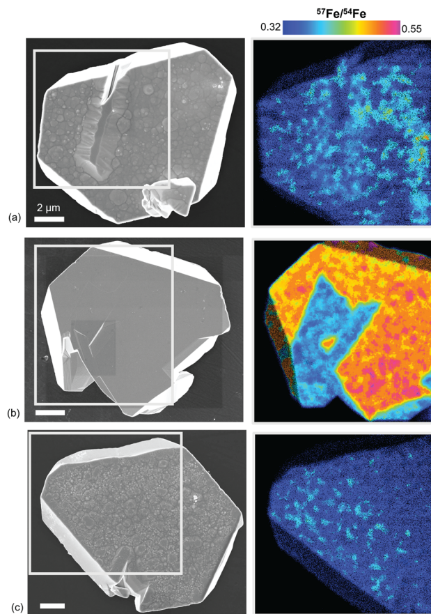
Fig. 5 Morphological characteristics shown by SEM and correlative NanoSIMS isotopic mapping on the (a) control ^{NA}\text{Fe(II)} -oxalate-hematite, (b) ^{57}\text{Fe(II)} -hematite, (c) ^{57}\text{Fe(II)} -oxalate-hematite samples.
