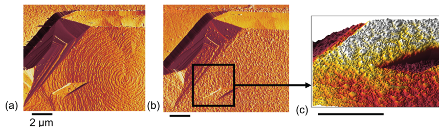
Fig. 4 Higher magnification AFM deflection image from the ^{57}\text{Fe(II)} -oxalate-hematite particle from Fig. 3d, showing the evolution of the basal and edge surfaces as well as an intergrowth feature (a) before and (b) after reaction. (c) A higher magnification and rotated 3D image from the region in panel b, highlighting the pyramidal microtopography. Scale bar is 2 \mu\text{m} .
