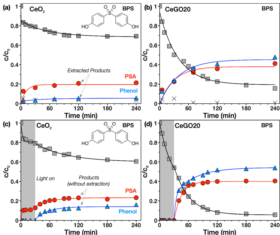
Fig. 6 Reactive adsorption of BPS on (a) CeO 2 and (b) CeO 2 nanoparticles grown on GO (representative sample CeGO20); solar-light enhanced photodecomposition of BPS on (c) CeO 2 and (d) sample CeGO20. Color coding: black squares – BPS concentration in solution, black crosses – BPS extracted from the surface of the catalyst, red circles – PSA and blue triangles – phenol (both extracted in the case of dark tests or released and analyzed directly in solution in photocatalytic tests).
