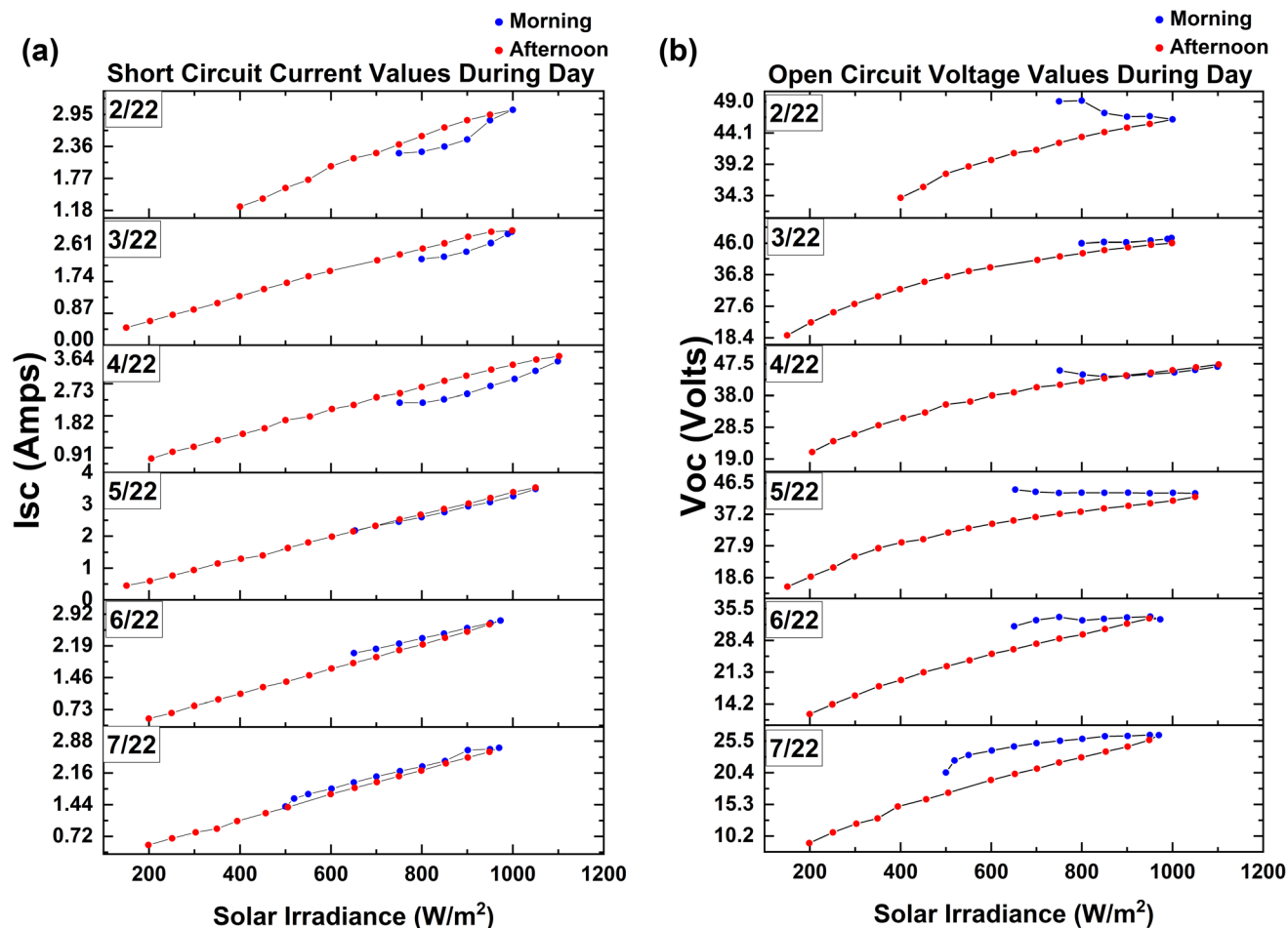
Fig. 8 Evidence of the light soaking phenomenon affecting the electrical characteristics of the solar farm behavior charge during the day for each month after a 3-month dark storage period.
