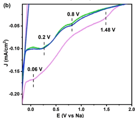
Fig. 2 (a) Cyclic voltammetry curves for the mixtures with 42 mol% NaFSI system at 1 st cycle. (b) The enlarged reduction process.
