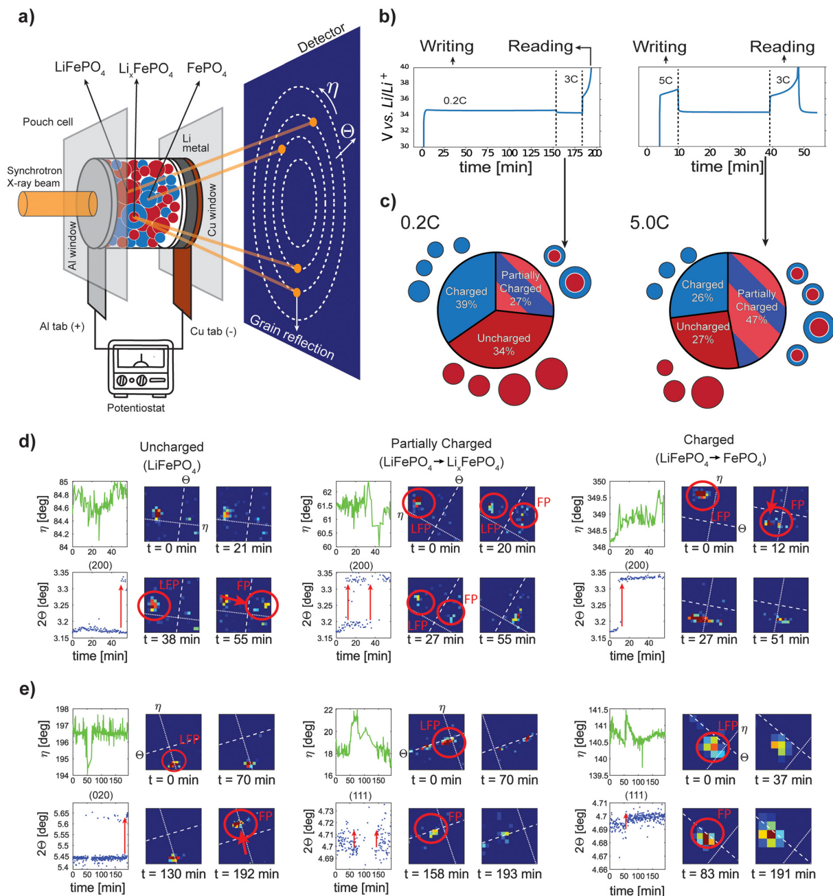
Fig. 2 Microbeam X-ray diffraction analysis. (a) Schematic of the microbeam X-ray diffraction experimental setup. (b) Measured voltage evolution during the microbeam X-ray diffraction operando experiments: 0.2C–3.0C and 5.0C–3.0C cycles, respectively. (c) Fractions of particles uncharged ( \text{LiFePO}_4 , red), charged ( \text{FePO}_4 , blue) and partially charged ( \text{Li}_x\text{FePO}_4 , striped) at the end of the resting writing steps of the 0.2C–3.0C and 5.0C–3.0C cycles, respectively. (d) Evolution of the (200) reflection during the 5.0C–3.0C cycle for three different tracked grains. (e) Evolution of the (111) and (020) reflections during the 0.2C–3.0C cycle for three different tracked grains. The left-hand graphs show the evolution of the maximum intensity point for the selected grain reflection along the 2\theta and \eta directions. The heatmaps show the detected grain reflection at different times.
