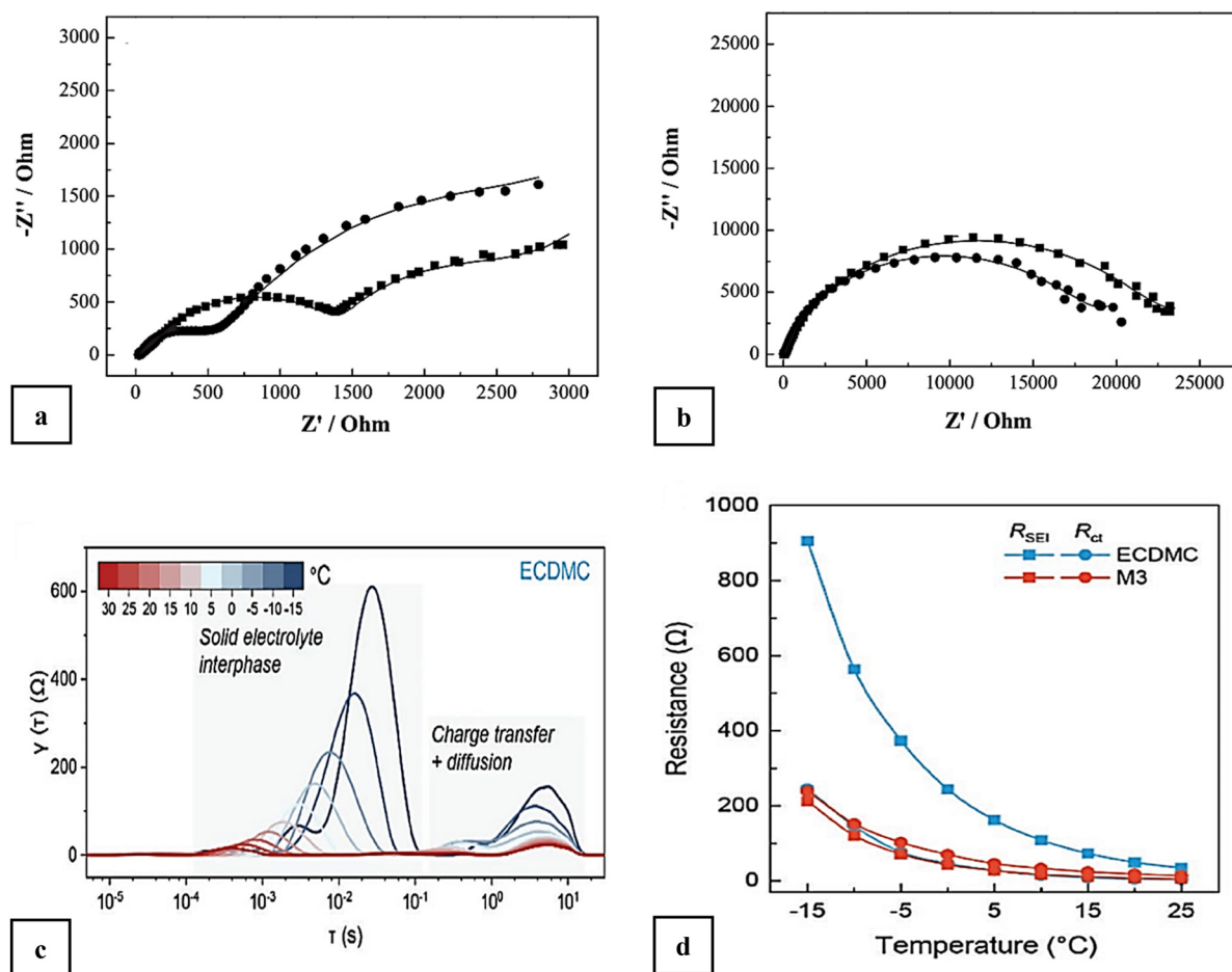
Fig. 6 EIS spectra of delithiated Li/MCMB cells using 1 M \text{LiPF}_6 in EC/PC/EMC (1:3:8 v/v/v) with fluoroethylene carbonate (FEC, squares) and without FEC (circles) at (a) -20^\circ\text{C} and (b) -40^\circ\text{C} . Reproduced with permission from ref. 34. (c) DRT analysis of the Nyquist plots for graphite electrodes at various temperatures using 1 M \text{LiPF}_6 in EC/DMC (3:7 v/v) electrolyte. Reproduced with permission from ref. 27. (d) R_{\text{SEI}} and R_{\text{ct}} values of graphite electrodes obtained from EIS fitting at different temperatures using various electrolytes. Reproduced with permission from ref. 27.
