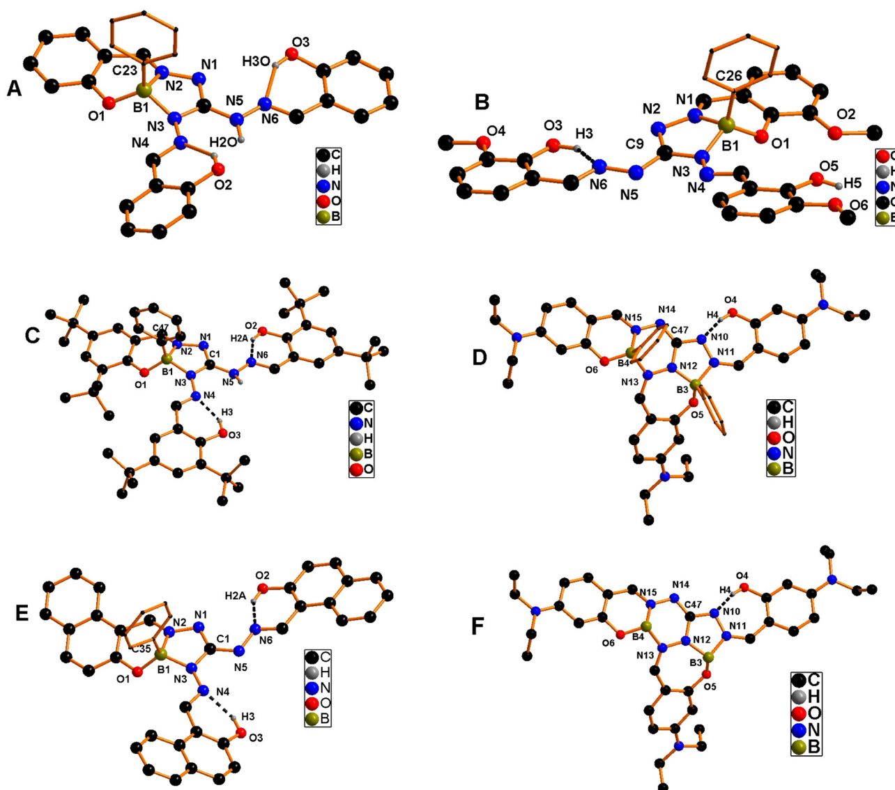
Fig. 1 (A–E) Molecular structure of compounds 6–10. (F). View of boron fused two six membered, one five membered and seven membered heterocycles of compound 9, here phenyl group on boron atoms are omitted for clarity.
