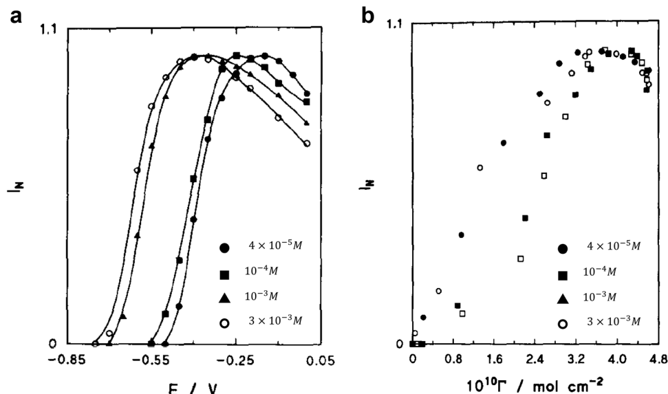
Fig. 50 (a) Plots of the intensity of the 1010\text{ cm}^{-1} band on the electrode potential ( E vs. SCE) for the varied bulk pyridine concentrations. (b) Data from panel a plotted versus surface concentration of pyridine \Gamma . Figures are adapted from ref. 119 with permission. Copyright 1991 Elsevier.
