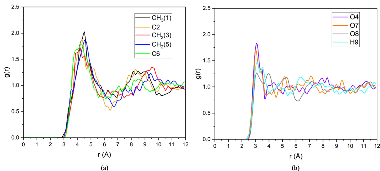
Fig. 4 Site–site intermolecular RDFs for the \text{C}(\text{CO}_2)\text{--levulinic acid} system: (a) \text{CH}_3(1) , C2, \text{CH}_2(3) , \text{CH}_2(5) and C6 groups of levulinic acid and (b) O4, O7, O8 and H9 groups of levulinic acid.
