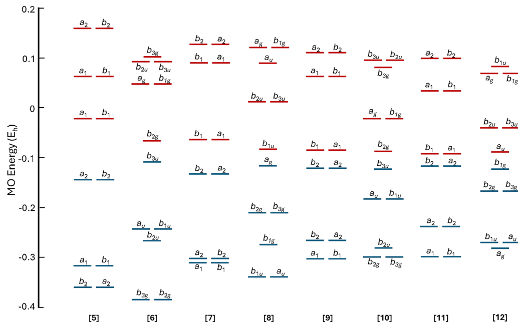
Fig. 2 The molecular orbital diagrams ( E in E_h ) of [n] -cyclacenes ( n = [5,12] ) in the range from (HOMO–5) to (LUMO+5) as computed at the CASSCF(12,12)/def2-TZVP level of theory. Occupied and vacant MO are in blue and red, respectively. Symmetry labels given are for D_{2h} (even n ) and C_{2v} (odd n ) point groups.
