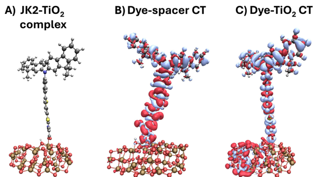
Fig. 9 Structure of the JK2-TiO 2 dye-semiconductor complex (panel A). Isosurface plot of the density differences for dye-spacer (panel B), and dye-TiO 2 (panel C) CT excitations of the JK2-TiO 2 complex computed with the FRZ-SGM method. The isosurface plot is obtained by using an isovalue of 0.0005 for the blue surface and -0.0005 for the red surface.
