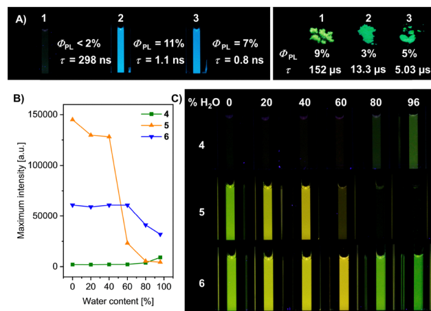
Fig. 2 (A) Photographs under 365 nm UV light, quantum yields ( \Phi_{\text{PL}} ) and amplitude-weighted average lifetimes ( \tau ) of compounds 1–3 in THF solution and the solid state. (B) Emission intensity of compounds 4–6 in water/THF mixtures. (C) Photographs of compounds 4–6 in water/THF mixtures under 365 nm UV light.
