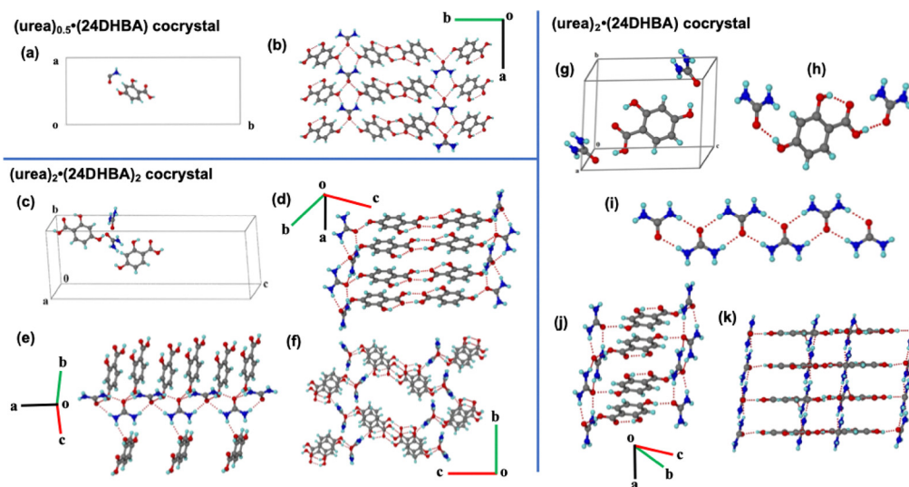
Fig. 1 Crystal packing and hydrogen bond interactions present in the variable stoichiometric cocrystals of urea with 24DHBA, respectively (a) and (b) (\text{urea})_{0.5} \cdot (\text{24DHBA}) ; (c)–(f) (\text{urea})_2 \cdot (\text{24DHBA})_2 and (g)–(k) (\text{urea})_2 \cdot (\text{24DHBA}) .
