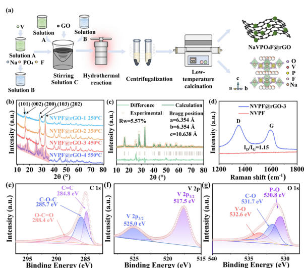
Fig. 1 (a) Production process and crystal structure of NVPF. (b) XRD patterns of NVPF@rGO at different temperatures. (c) Rietveld's refinement of NVPF@rGO-3. (d) Raman curves of NVPF@rGO-3 and NVPF. XPS spectra of (e) C 1s, (f) V 2p, and (g) O 1s.
