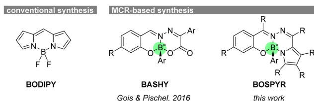
Fig. 1 BODIPY dyes accessible through conventional synthesis vs. BASHY dyes and BOSPYR dyes (this work) through MCR approach.
