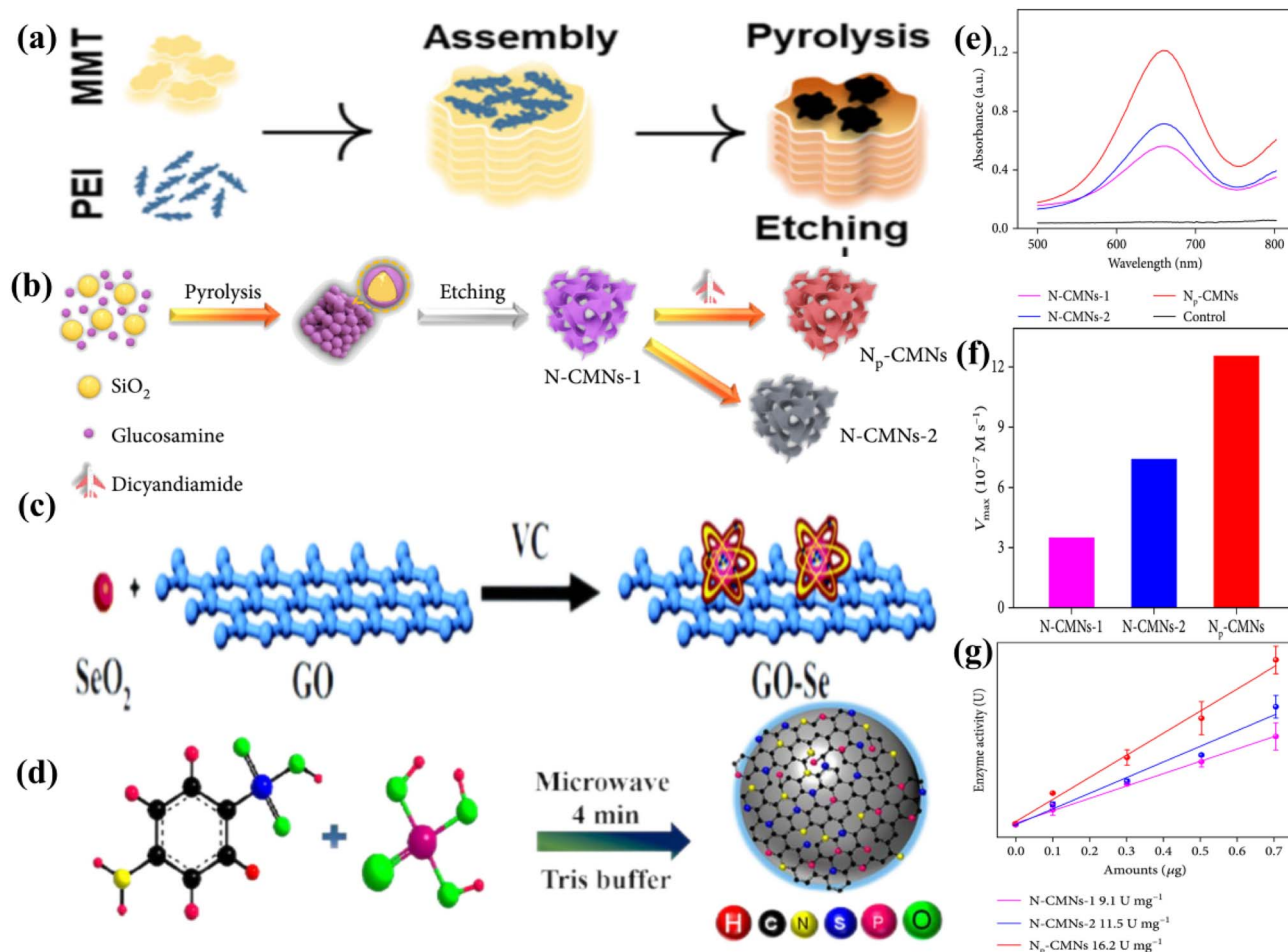
Fig. 3 Synthesis of (a) N-doped carbon sheets via strong electrostatic attraction between MMT and PEI, (b) N-CMN-1, (c) GO-Se nanocomposites, and (d) NSP-CQDs. (e) UV-vis absorption spectra of POD-like catalytic oxidation with N-CMN-1, (f) V_{\text{max}} ( \text{H}_2\text{O}_2 substrate) and (g) specific activity (SA) of N-CMN-1.
