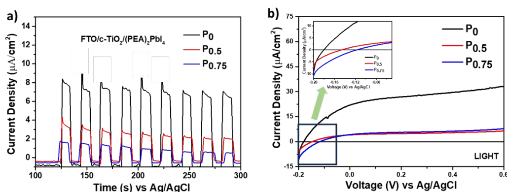
Fig. 4: a) The chronoamperometric and b) LSV curves (over c-TiO 2 ) of P 0 , P 0.5 , and P 0.75 compositions. [P 0 = pristine (PEA) 2 PbI 4 , P 0.5 = 0.5 mg PCBM mixed in 1 ml (PEA) 2 PbI 4 perovskite precursor, and P 0.75 = 0.75 mg PCBM mixed in 1 ml (PEA) 2 PbI 4 perovskite precursor solution.]
