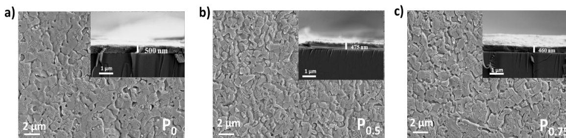
Fig. 2: Surface and cross-sectional images ( given in the inset) of a) P_0 , b) P_{0.5} , c) P_{0.75} compositions. [ P_0 = pristine (\text{PEA})_2\text{PbI}_4 , P_{0.5} = 0.5 mg PCBM mixed in 1 ml (\text{PEA})_2\text{PbI}_4
