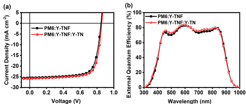
Fig. 3 (a) J - V plots of the PM6:Y-TNF:Y-TN-based OSCs (1:1:0 and 1:1:0.1, w/w/w) with 0.25% DIO additive, and a TA treatment at 100 ^{\circ}\text{C} for 5 min under an illumination of AM 1.5 G, 100 \text{mW cm}^{-2} , and (b) EQE curves of the corresponding OSCs.
