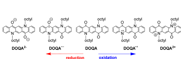
Scheme 2 Representation of oxidised and reduced forms of DOQA.
