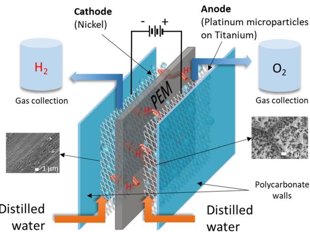
Fig. 1 Schematic diagram of the experimental electrolyzer.
