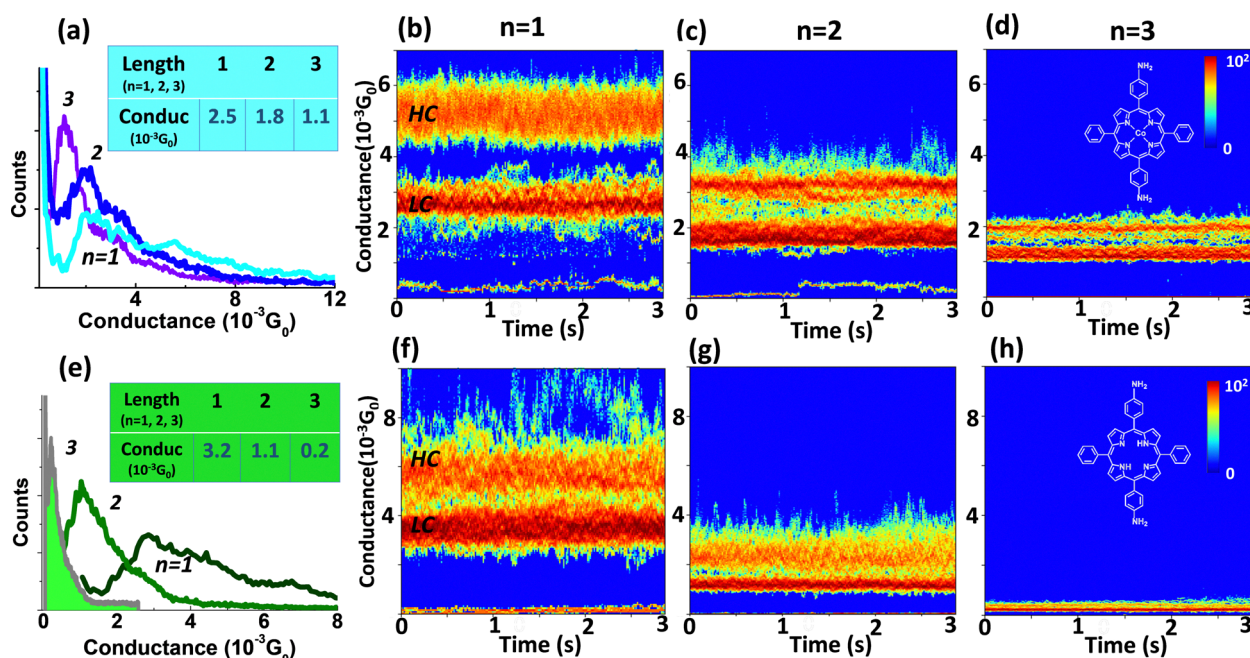
Fig. 3 Combined STM-bj histograms: (a) Au-[CoTPP] n -Au and (e) Au-[TPP] n -Au SMJs ( n = 1-3 ). Inset tables indicate the conductance values. (b)–(d), (f)–(h) G_{\text{time}} 2D heat maps for both SMJs with different junction lengths ( n = 1-3 ).
