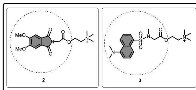
Fig. 6 Molecular structure of compound 2 and 3 .
