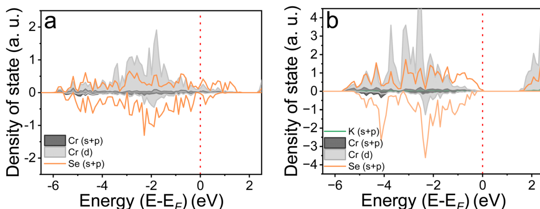
Fig. 1 The partial density of states of the valence bands of (a) \text{CrSe}_2 and (b) \text{KCrSe}_2 . The Fermi energy E_F is given by a dashed line.
