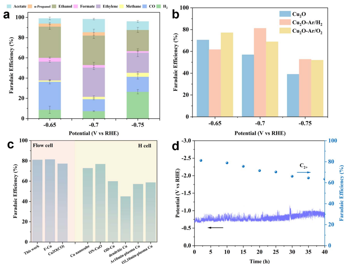
Fig. 3 ECR performance of the as-prepared catalysts. (a) The reduced product distribution of \text{CO}_2 for \text{Cu}_2\text{O–Ar/H}_2 at different cathodic potentials under ECR. (b) The FEs for \text{C}_{2+} products on the as-synthesized samples. (c) Comparisons of the FE values for \text{C}_{2+} products between \text{Cu}_2\text{O–Ar/H}_2 and other recently reported plasma-treated Cu-based catalysts. The summary of the specific ECR performance of catalysts is presented in Table S1.† (d) The stability test of \text{Cu}_2\text{O–Ar/H}_2 at a current density of 100 \text{mA cm}^{-2} using a flow cell.
