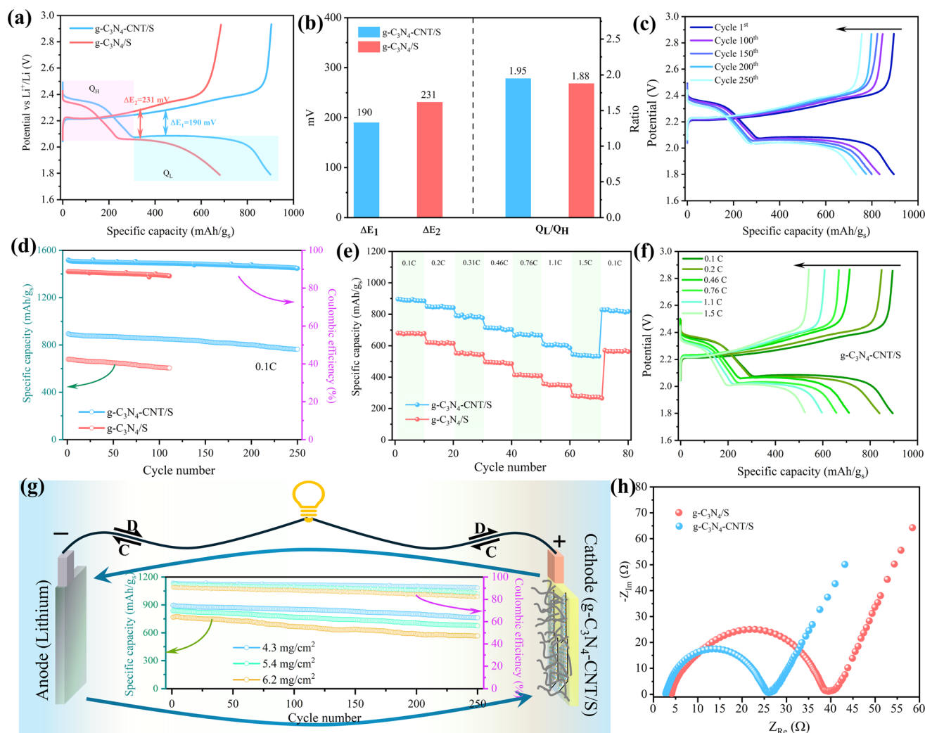
Fig. 6 (a) Initial charge–discharge curves for the g\text{-C}_3\text{N}_4/\text{S} and g\text{-C}_3\text{N}_4\text{-CNT/S} cathodes at 0.1C, (b) the capacity contribution of Q_{\text{H}} , Q_{\text{L}} , and the Q_{\text{L}}/Q_{\text{H}} ratio of g\text{-C}_3\text{N}_4\text{-CNT/S} and g\text{-C}_3\text{N}_4/\text{S} at 0.1C, (c) galvanostatic charge–discharge profiles of the g\text{-C}_3\text{N}_4\text{-CNT/S} cathode for 250 cycles, (d) cycle performance and coulombic efficiency of g\text{-C}_3\text{N}_4/\text{S} and g\text{-C}_3\text{N}_4\text{-CNT/S} cathodes for 110 and 250 cycles, respectively, (e) rate capabilities of g\text{-C}_3\text{N}_4/\text{S} and g\text{-C}_3\text{N}_4\text{-CNT/S} cathodes under various current densities, (f) galvanostatic charge–discharge profiles of the g\text{-C}_3\text{N}_4\text{-CNT/S} cathode at different current densities, (g) cycle performance of the g\text{-C}_3\text{N}_4\text{-CNT/S} cathode with varied sulfur loading for 250 cycles at 0.1C and (h) EIS spectra of the freshly prepared uncycled cell.
