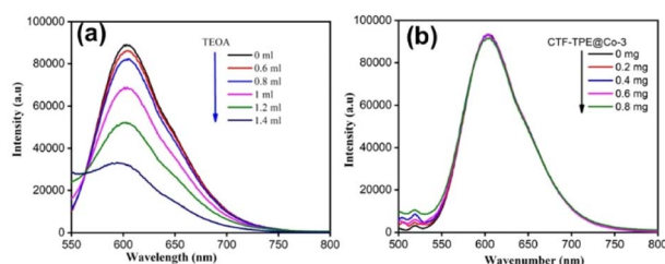
Fig. 7 (a) Fluorescence spectra of [Ru(bpy) 3 ] 2+ in the presence of TEOA. (b) Fluorescence spectra of [Ru(bpy) 3 ] 2+ in the presence of CTF-TPE@Co-3.
