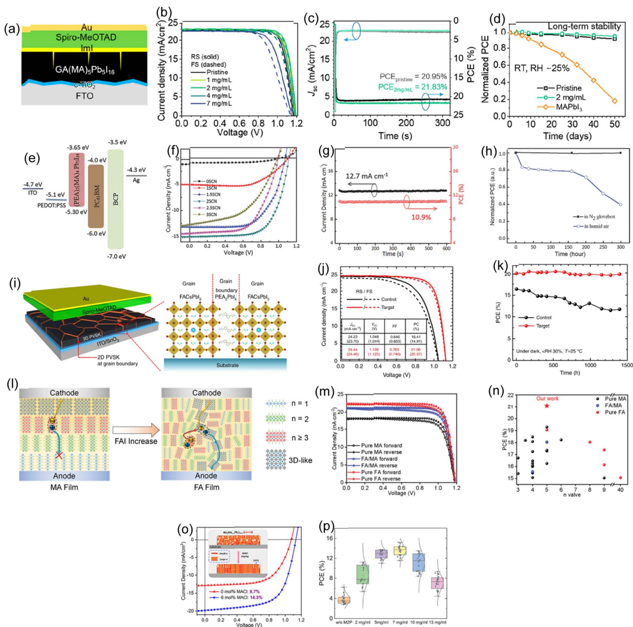
Fig. 4 (a) The quasi-2D ACI \text{GA(MA)}_n\text{PbI}_{3n+1} ( n = 5 ) based PSC device structure. (b) J - V curves of PSCs with and without (pristine) Iml treatment in both forward and reverse scans. (c) PSC's stabilized power output was measured at the MPP at a bias voltage of 0.948 V. The untreated (pristine) and treated samples contained 2 \text{ mg mL}^{-1} Iml. (d) Stability of PSCs with and without ( 2 \text{ mg mL}^{-1} ) Iml treatment and PSCs based on \text{MAPbI}_3 . (a)–(d) Reproduced with permission. 68 Copyright 2022, ACS. (e) PVSC device energy band alignment, (f) J - V curves of the devices with varying \text{NH}_4\text{SCN} concentrations, (g) PSCs' photocurrent, (h) PSC devices' stability was tested in both an \text{N}_2 glove box and an environment with a humidity of 55% based on the (\text{PEA})_2(\text{MA})_4\text{PbI}_5 ( n = 5 ) perovskite film. (e)–(h) Reproduced with permission. 69 Copyright 2018, Wiley. (i) Device schematics that use a polycrystalline 3D perovskite film with 2D perovskites at the grain boundaries. (j) J - V curves. (k) Evolution of the PCE of the target and control. The devices were kept in a controlled-humidity environment that was dark. (l)–(k) Reproduced with permission. 148 Copyright 2018, Nature. (l) MA and FA-based schematics of 2D perovskites' crystal orientation and phase distribution in oblique and graded vertical alignments. (m) J - V curves for the best pure MA, FA/MA, and pure FA devices while scanning forward and backward. (n) High-efficiency, low-dimensional perovskite solar cell PCE is summarised. (l)–(n) Reproduced with permission. 70 Copyright 2022, Wiley. (o) J - V curves for 0 and 6 mol% MACl PSC champion devices. The inset schematic shows how MACl doping changes stacked perovskite films. Reproduced with permission. 149 Copyright 2020, ACS. (p) PCE statistics of PSCs that did not contain spiro-OMeTAD, broken down according to the different conditions of M2P precursor solution. Reproduced with permission. 150 Copyright 2020, Wiley.
