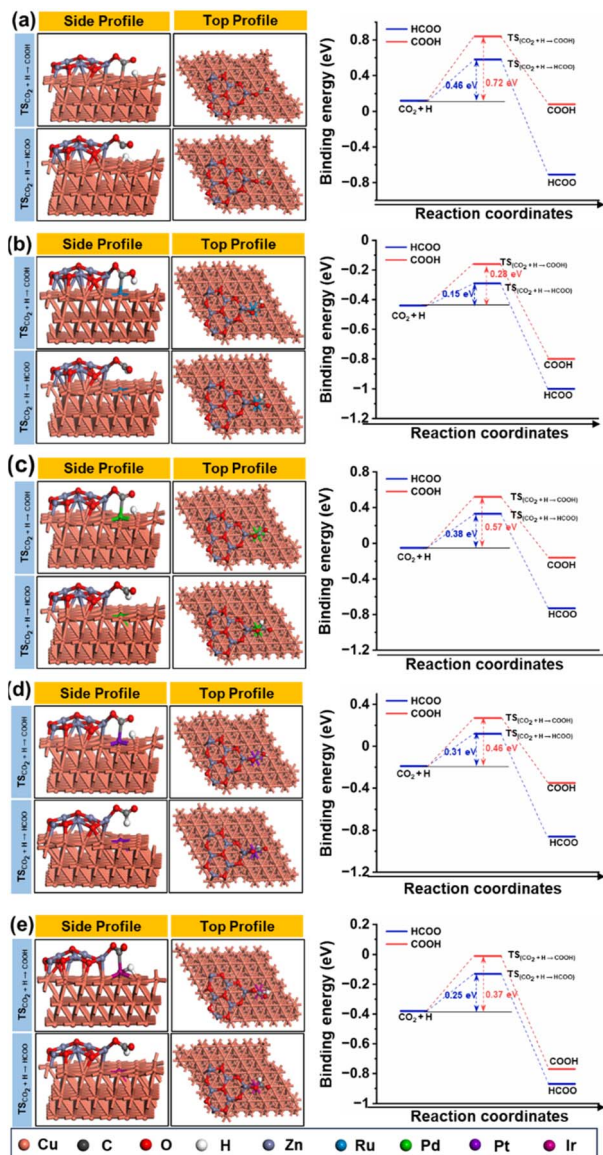
Fig. 15 The geometry optimised structure of the transition state during conversion of CO 2 + H to HCOO and COOH and associated energy profile diagrams for (a) CZ, (b) Ru-CZ, (c) Pd-CZ, (d) Pt-CZ and (e) Ir-CZ.
