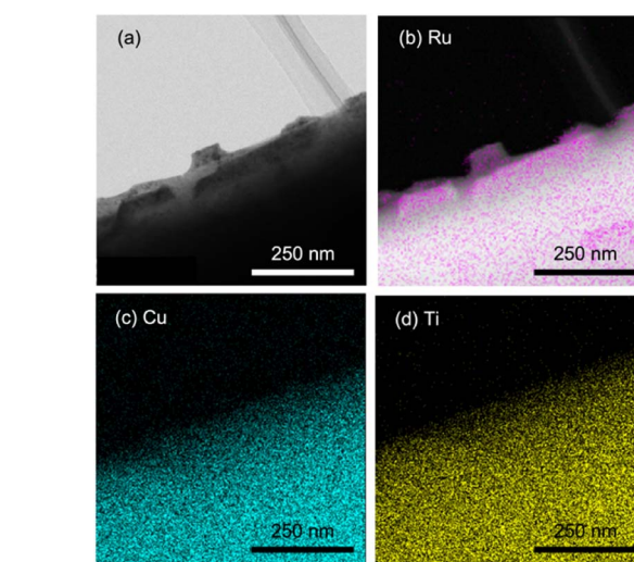
Fig. 6 (a) TEM image and (b–d) STEM-EDS images of Ru(100\% \text{ MeOH})/CLTO .
