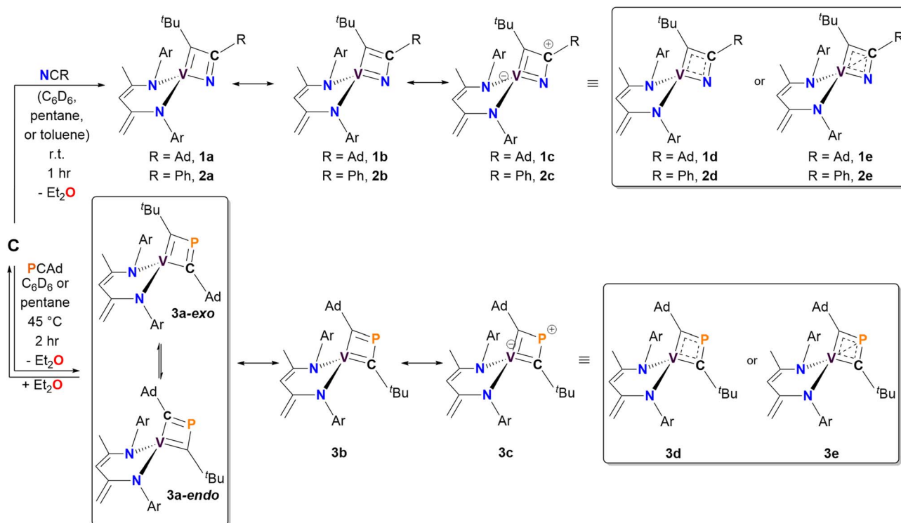
Scheme 1 Synthesis of complexes 1 – 3 via the [2+2]-cycloaddition of the vanadium alkylidyne C with pnictogen-containing alkynes \text{Pn}\equiv\text{CR} ( \text{Pn} = \text{N} , \text{R} = \text{Ad} or \text{Ph} ; \text{Pn} = \text{P} , \text{R} = \text{Ad} ). Potential resonance structures and charge delocalized structures for each complex are also illustrated.
