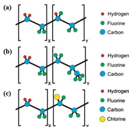
Fig. 7 Schematic diagram showing the repeat units of (a) P(VDF-TrFE); (b) P(VDF-HFP); and (c) P(VDF-CTFE). This figure has been reproduced from ref. 75 with permission from Elsevier, copyright 2014.
