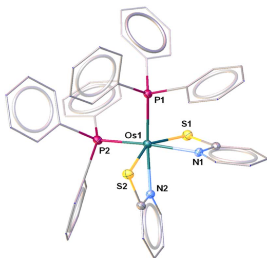
Fig. 1 Molecular structure and labelling diagram of 2b . Selected bond lengths ( \text{\AA} ) and bond angles ( ^\circ ) of 2b : Os1–N1 2.143(3), Os1–N2 2.134(3), Os1–P1 2.2887(10), Os1–P2 2.2993(10), Os1–S1 2.4318(10), Os1–S2 2.4257(10); S2–Os1–S1 150.98(4), and N2–Os1–N1 80.11(13).
