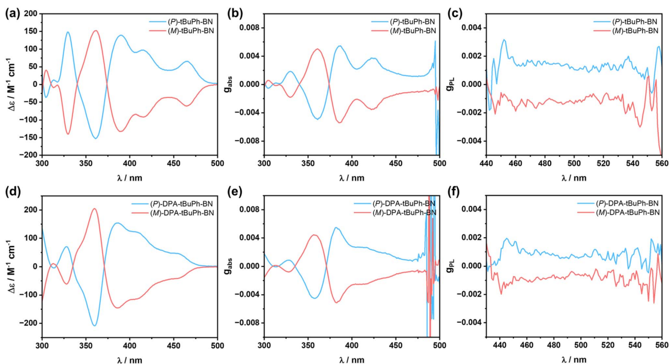
Fig. 6 (a) CD spectra and (b) g_{\text{abs}} values of t BuPh-BN recorded in 5 \times 10^{-6} \text{ mol L}^{-1} toluene solution. (c) g_{\text{PL}} values of t BuPh-BN recorded in 10^{-5} \text{ mol L}^{-1} THF solution. (d) CD spectra and (e) g_{\text{abs}} values of DPA- t BuPh-BN recorded in 5 \times 10^{-6} \text{ mol L}^{-1} toluene solution. (f) g_{\text{PL}} values of DPA- t BuPh-BN recorded in 10^{-5} \text{ mol L}^{-1} THF solution.
