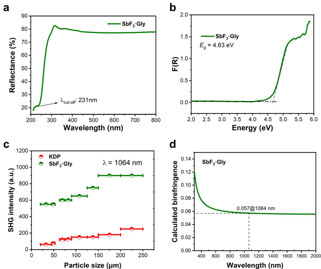
Fig. 2 The linear and nonlinear optical properties of \text{SbF}_3\cdot\text{Gly} . (a) The UV-vis diffuse reflectance spectrum and (b) optical band gap ( E_g ) determined using the Kubelka–Munk equation. (c) Particle size-dependent powder SHG efficiency. (d) Calculated birefringence.
