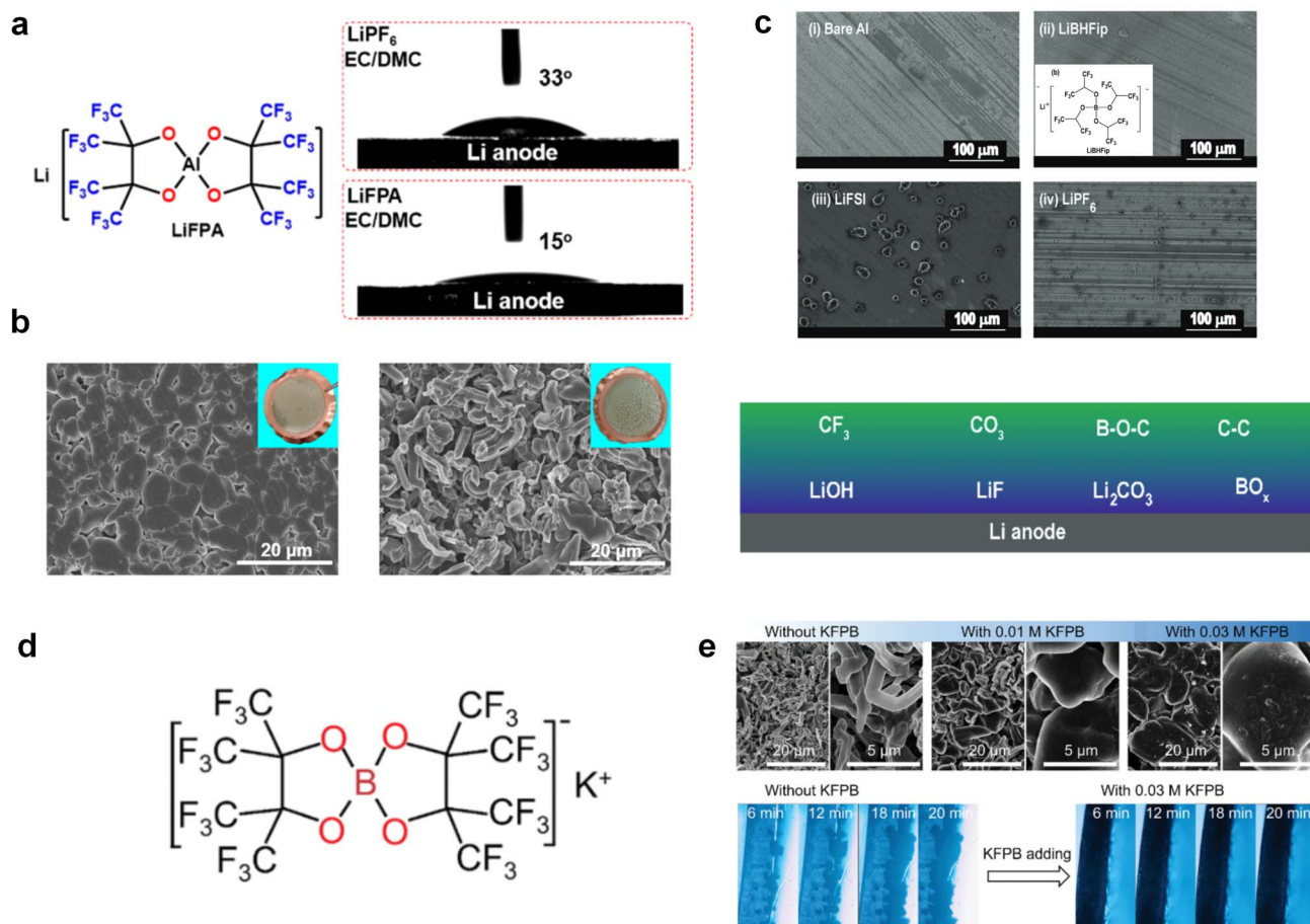
Fig. 13 Salt designs. (a) Contact angle of 1 M \text{LiPF}_6 -EC/DMC and 1 M \text{LiFPA} -EC/DMC to Li anode. (b) Morphology of deposited Li on Cu foil using 1 M \text{LiFPA} -EC/DMC and 1 M \text{LiPF}_6 -EC/DMC at a current density of 0.5 \text{ mA cm}^{-2} for 16 h. Insets are optical images of deposited Li on Cu foil. Reproduced with permission. Copyright © 2022 American Chemical Society. (c) Schematic representation of the species distribution in the Li electrode SEI. Reproduced with permission. Copyright © 2021 WILEY-VCH. (d) Molecular structure of KFPB. (e) Typical SEM images of deposited Li in BE electrolyte without and with 0.01/0.03 m KFPB ( 0.5 \text{ mA cm}^{-2} and 4 \text{ mA h cm}^{-2} ). In situ optical microscopy observations of Li plating at a current density of 5 \text{ mA cm}^{-2} in BE and BE with 0.03 m KFPB. Reproduced with permission. Copyright © 2023 WILEY-VCH.
