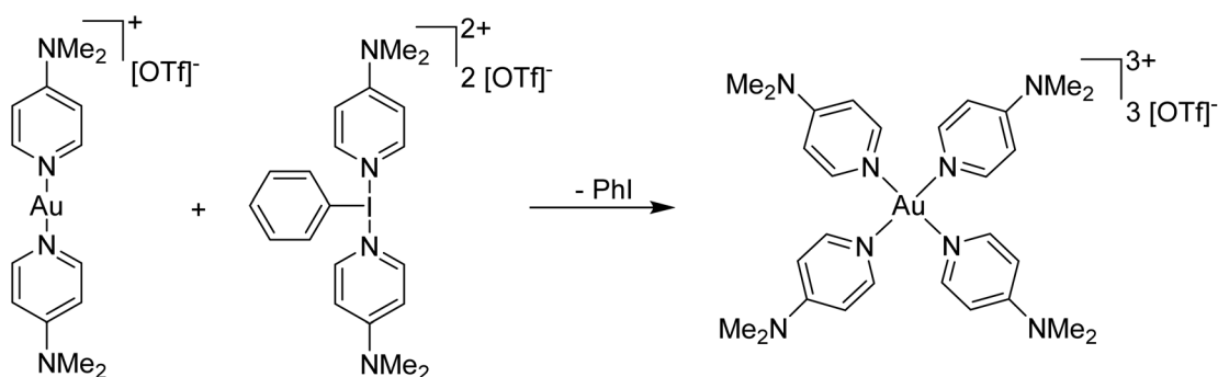
Scheme 3 Generation of a homoleptic Au(III) trication using a Weiss' reagent, [PhI(4-DMAP) 2 ][OTf].
