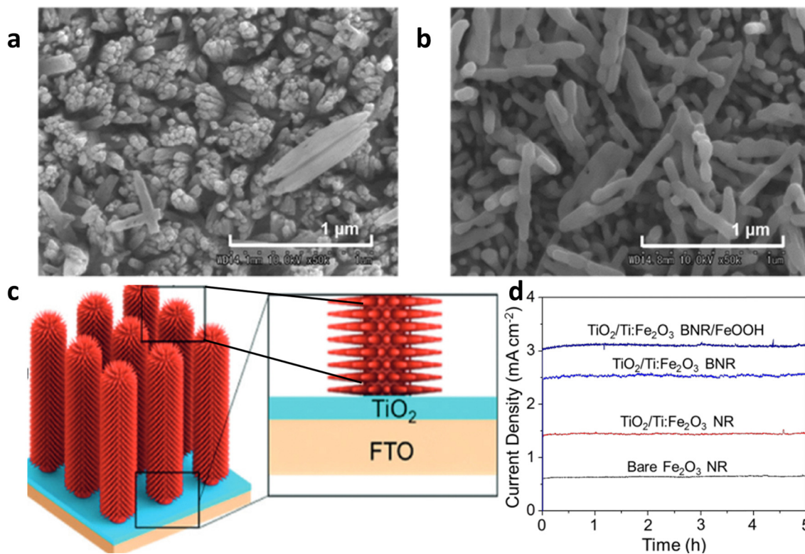
Fig. 13 Impact of underlayer TiO 2 . (a) Hematite grown on FTO. (b) Hematite grown on TiO 2 -coated FTO. Reprinted with permission from ref. 112, Copyright 2023 American Chemical Society. (c) Decoration of the TiO 2 layer between the branched hematite nanorod photoanode and FTO substrate for the synthesis of BNR. (d) Stability curve of the bare nanorod hematite photo anode with or without a branch, TiO 2 modification layer, and the cocatalyst. Reproduced from ref. 83 with permission from John Wiley and Sons, copyright 2017.
